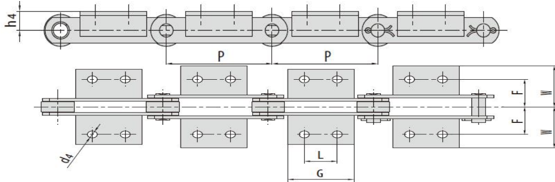
M系列带附板输送链 Conveyor chains with attachments (M series)
